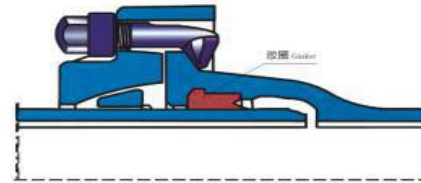
自锚接口 Self-restrained Joint pipe
